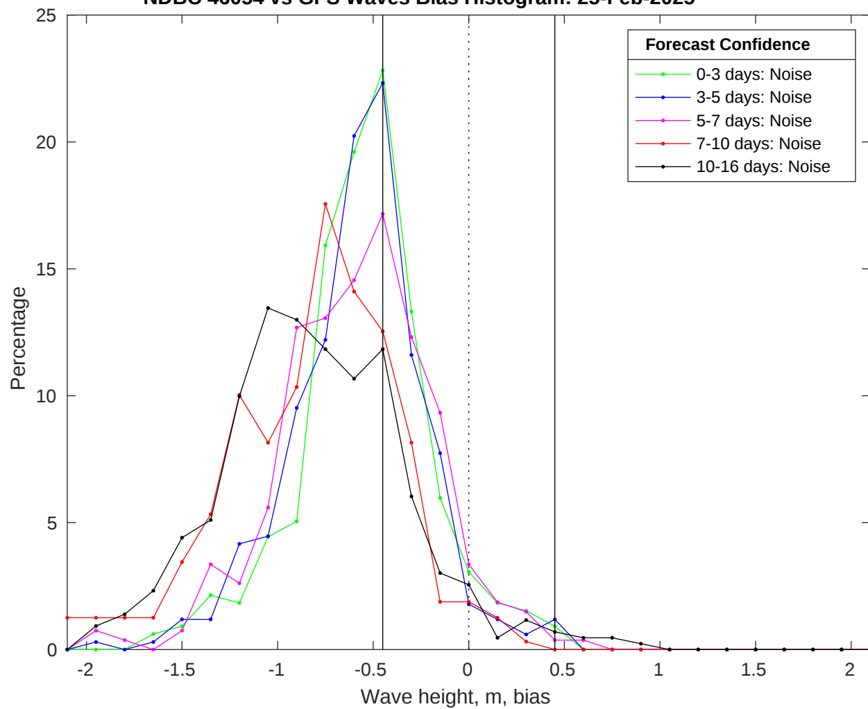
NDBC 46054 vs GFS Waves Bias Histogram: 25-Feb-2025
