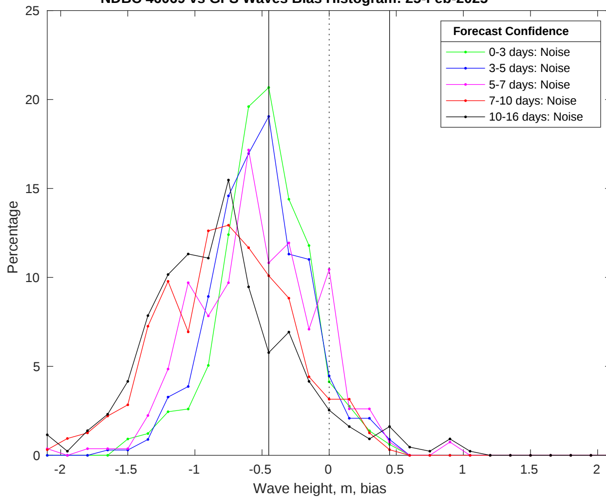
NDBC 46069 vs GFS Waves Bias Histogram: 25-Feb-2025
