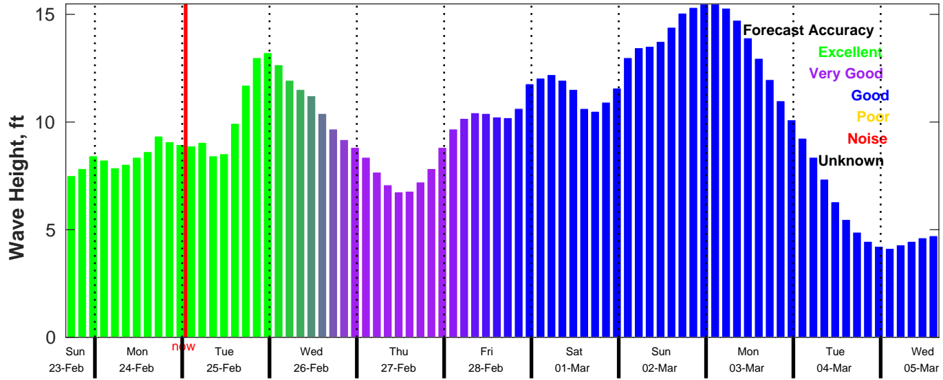
CMEMS Wave Forecast for NDBC 46069 from 23-Feb-2025 16:00:00 to 05-Mar-2025 16:00:00
