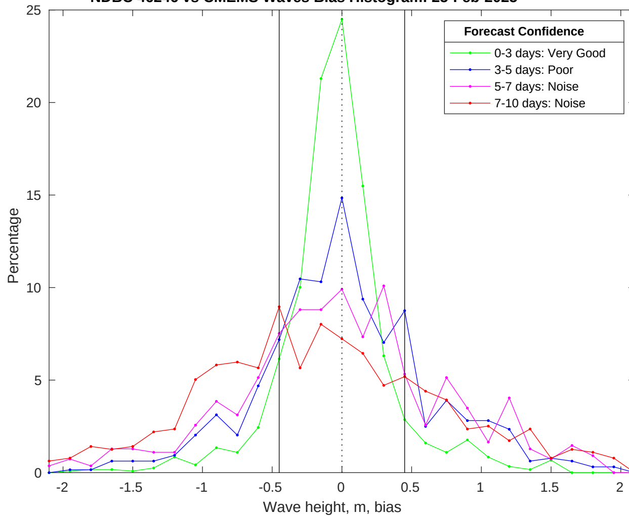
NDBC 46246 vs CMEMS Waves Bias Histogram: 25-Feb-2025
