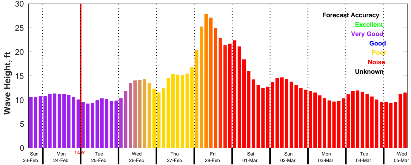
CMEMS Wave Forecast for NDBC 46246 from 23-Feb-2025 15:00:00 to 05-Mar-2025 15:00:00
