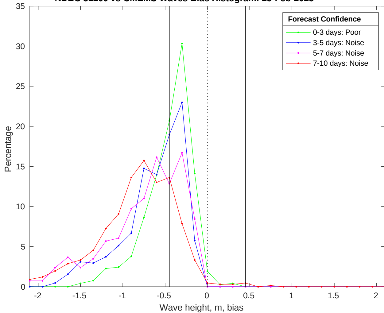
NDBC 51209 vs CMEMS Waves Bias Histogram: 25-Feb-2025
