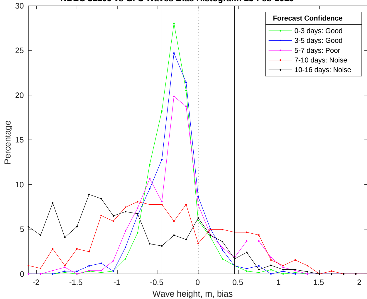
NDBC 51209 vs GFS Waves Bias Histogram: 25-Feb-2025
