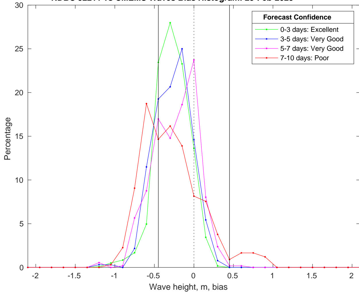
NDBC 52211 vs CMEMS Waves Bias Histogram: 25-Feb-2025
