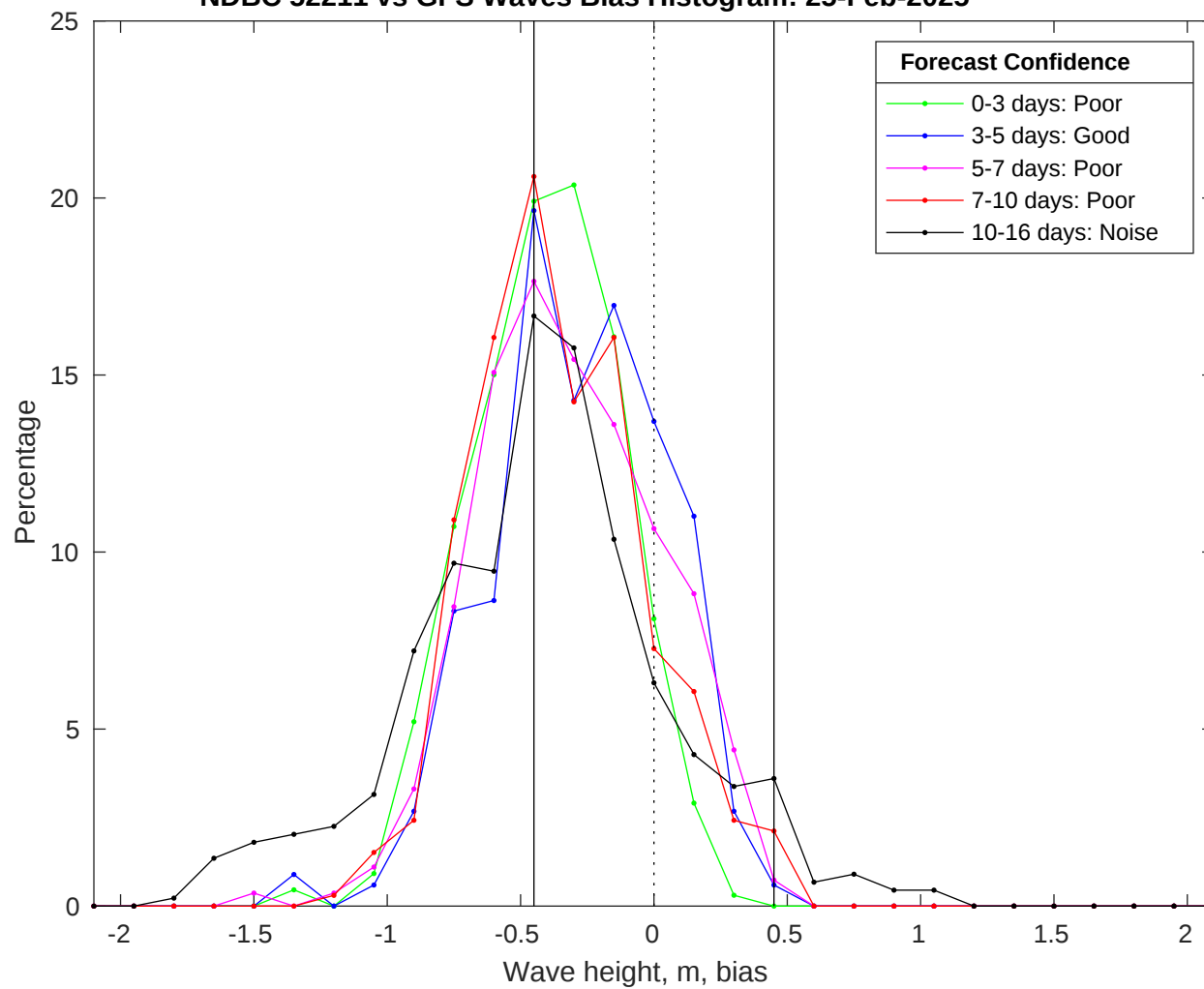
NDBC 52211 vs GFS Waves Bias Histogram: 25-Feb-2025
