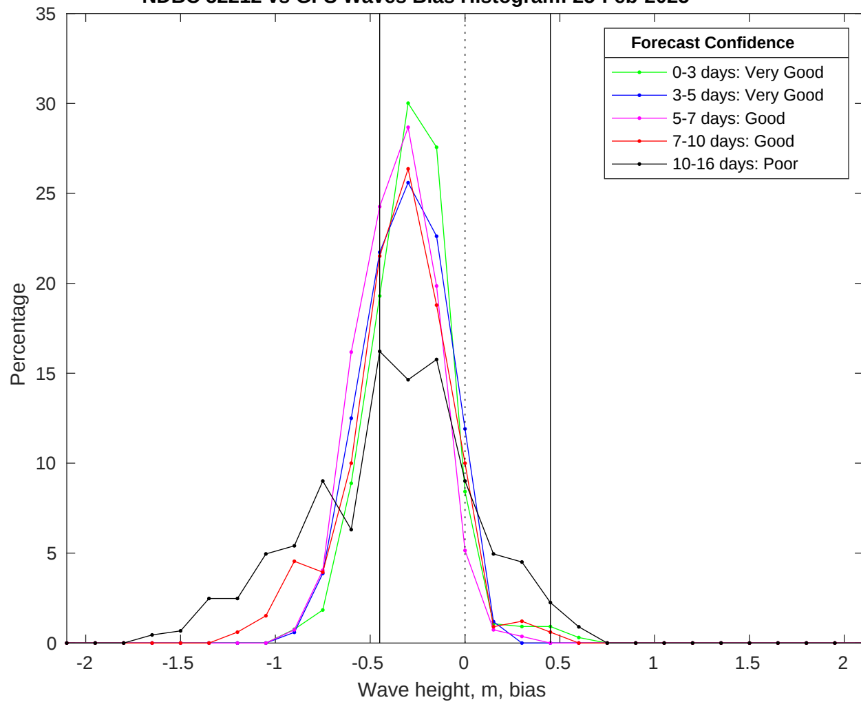
NDBC 52212 vs GFS Waves Bias Histogram: 25-Feb-2025
