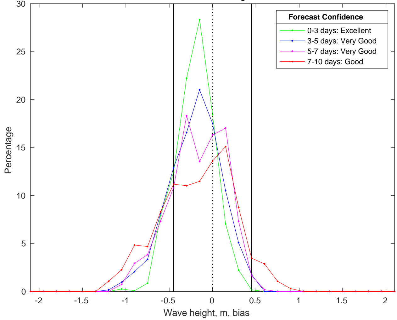
NDBC 52213 vs CMEMS Waves Bias Histogram: 25-Feb-2025
