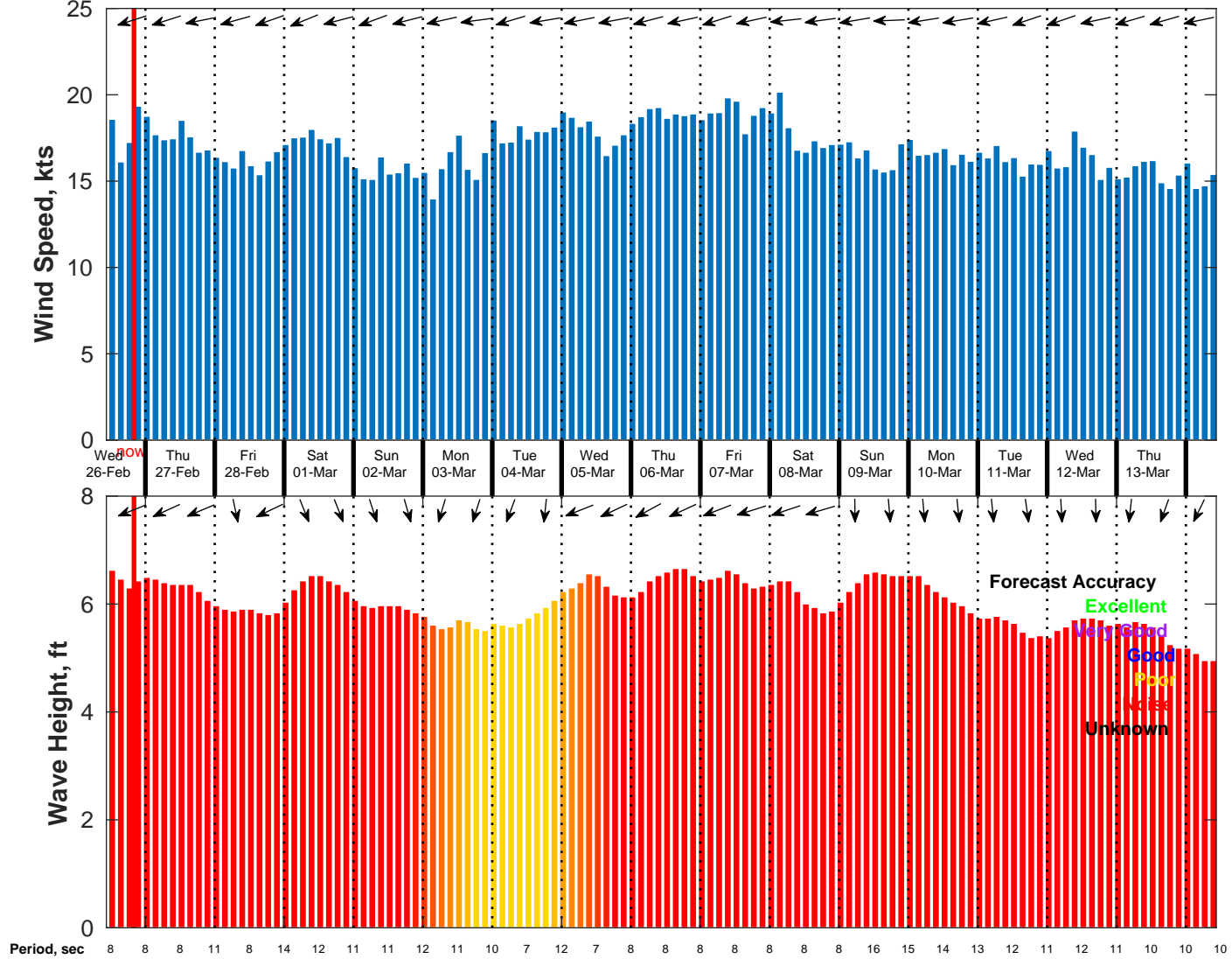
Wind & Wave Forecast for NDBC 52213 from 25-Feb-2025 11:00:00 to 13-Mar-2025 11:00:00
