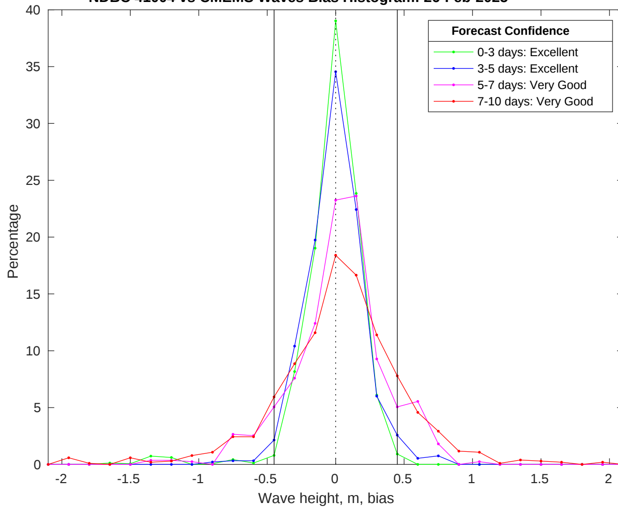
NDBC 41004 vs CMEMS Waves Bias Histogram: 26-Feb-2025
