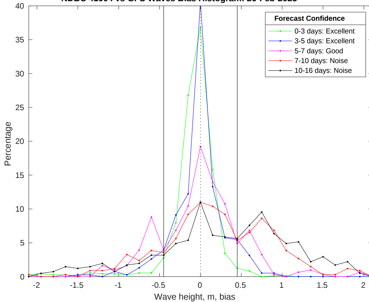
NDBC 41004 vs GFS Waves Bias Histogram: 26-Feb-2025
