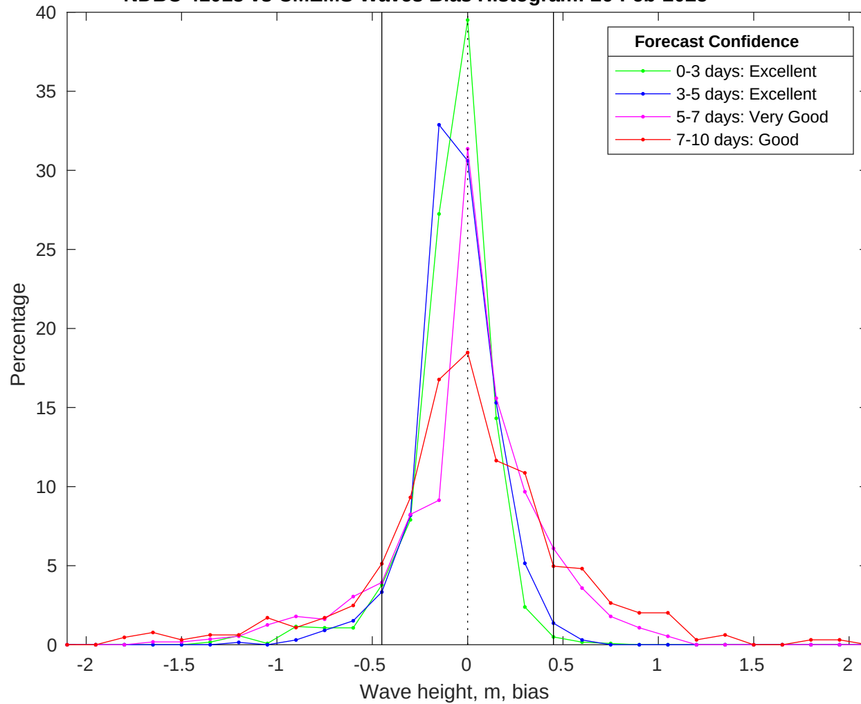
NDBC 41013 vs CMEMS Waves Bias Histogram: 26-Feb-2025
