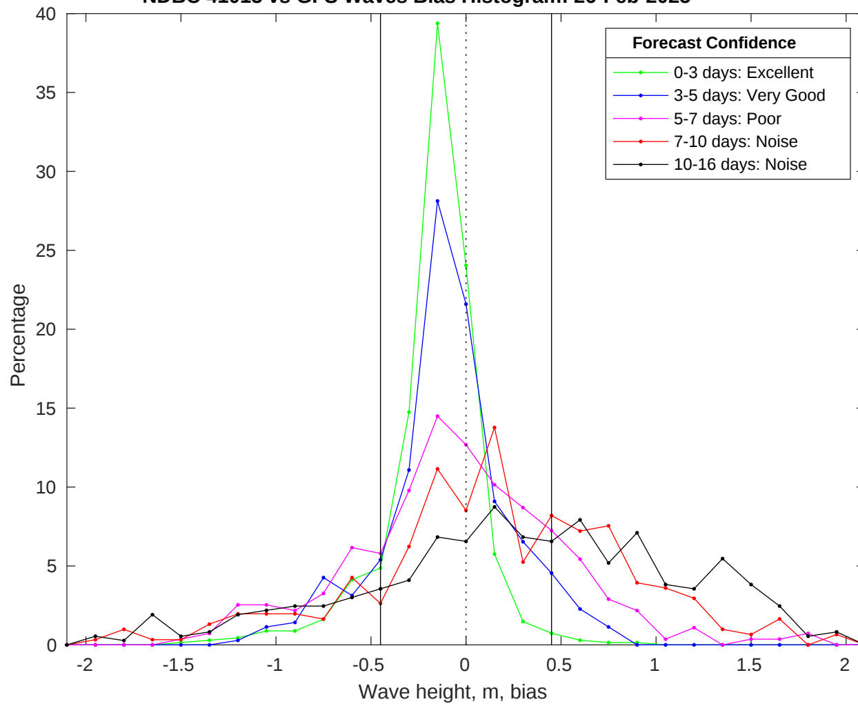
NDBC 41013 vs GFS Waves Bias Histogram: 26-Feb-2025
