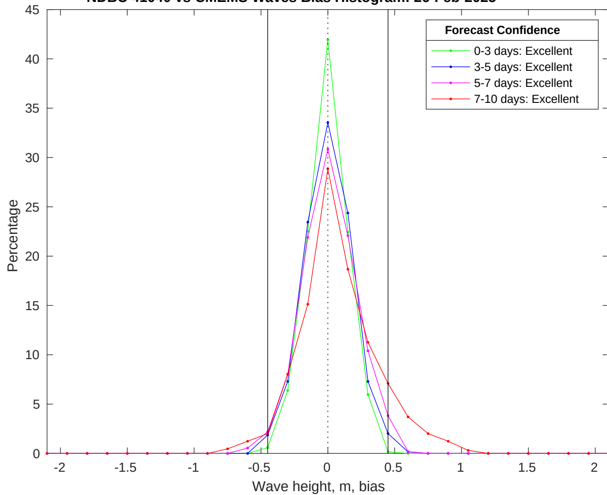
NDBC 41040 vs CMEMS Waves Bias Histogram: 26-Feb-2025
