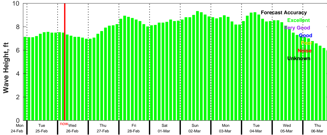
CMEMS Wave Forecast for NDBC 41040 from 24-Feb-2025 21:00:00 to 06-Mar-2025 21:00:00
