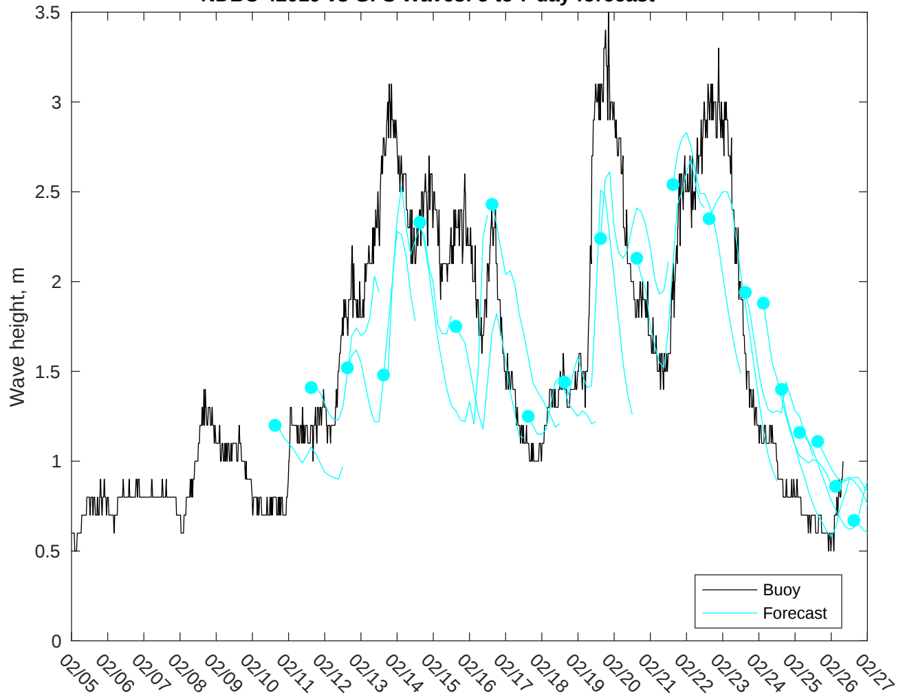
NDBC 42019 vs GFS Waves: 5 to 7 day forecast
