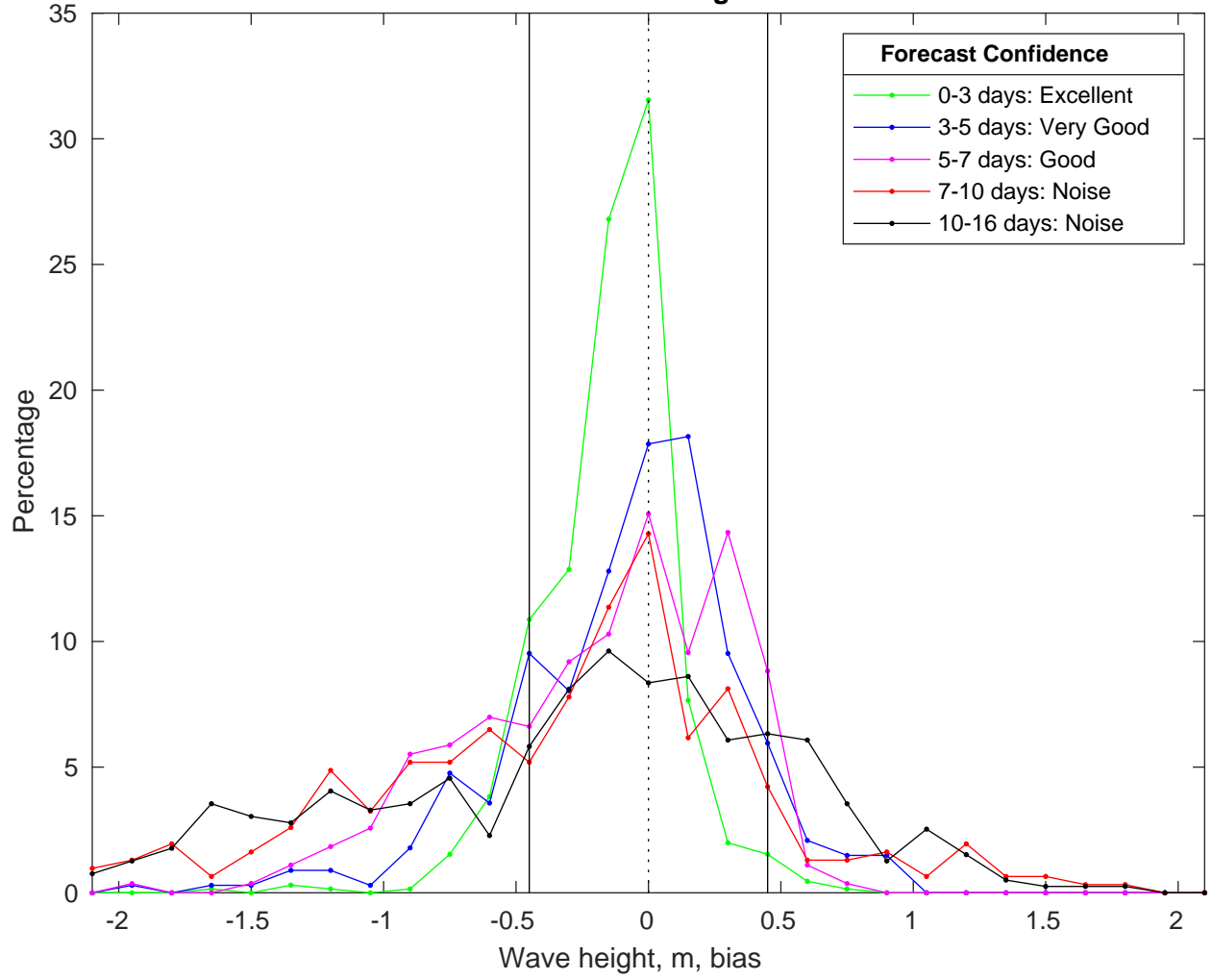
NDBC 42019 vs GFS Waves Bias Histogram: 26-Feb-2025
