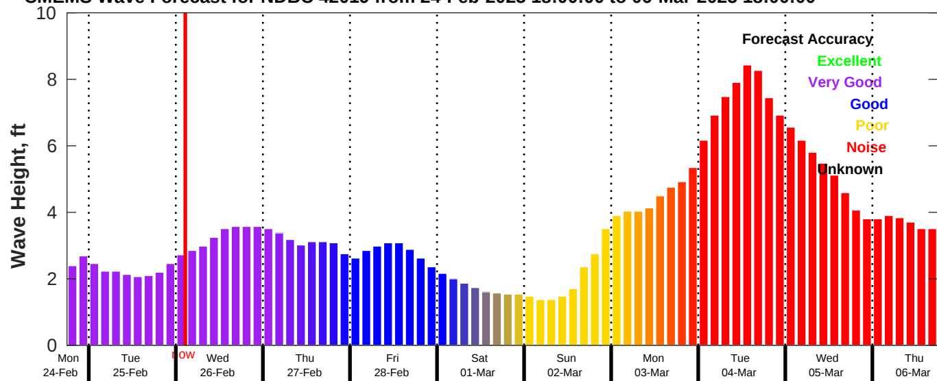
CMEMS Wave Forecast for NDBC 42019 from 24-Feb-2025 18:00:00 to 06-Mar-2025 18:00:00
