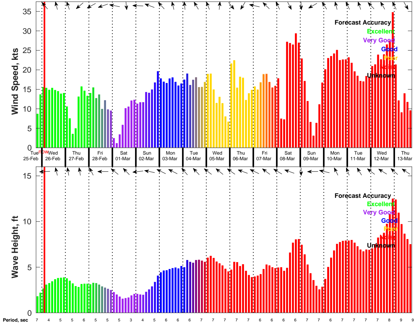
Wind & Wave Forecast for NDBC 42019 from 25-Feb-2025 18:00:00 to 13-Mar-2025 18:00:00
