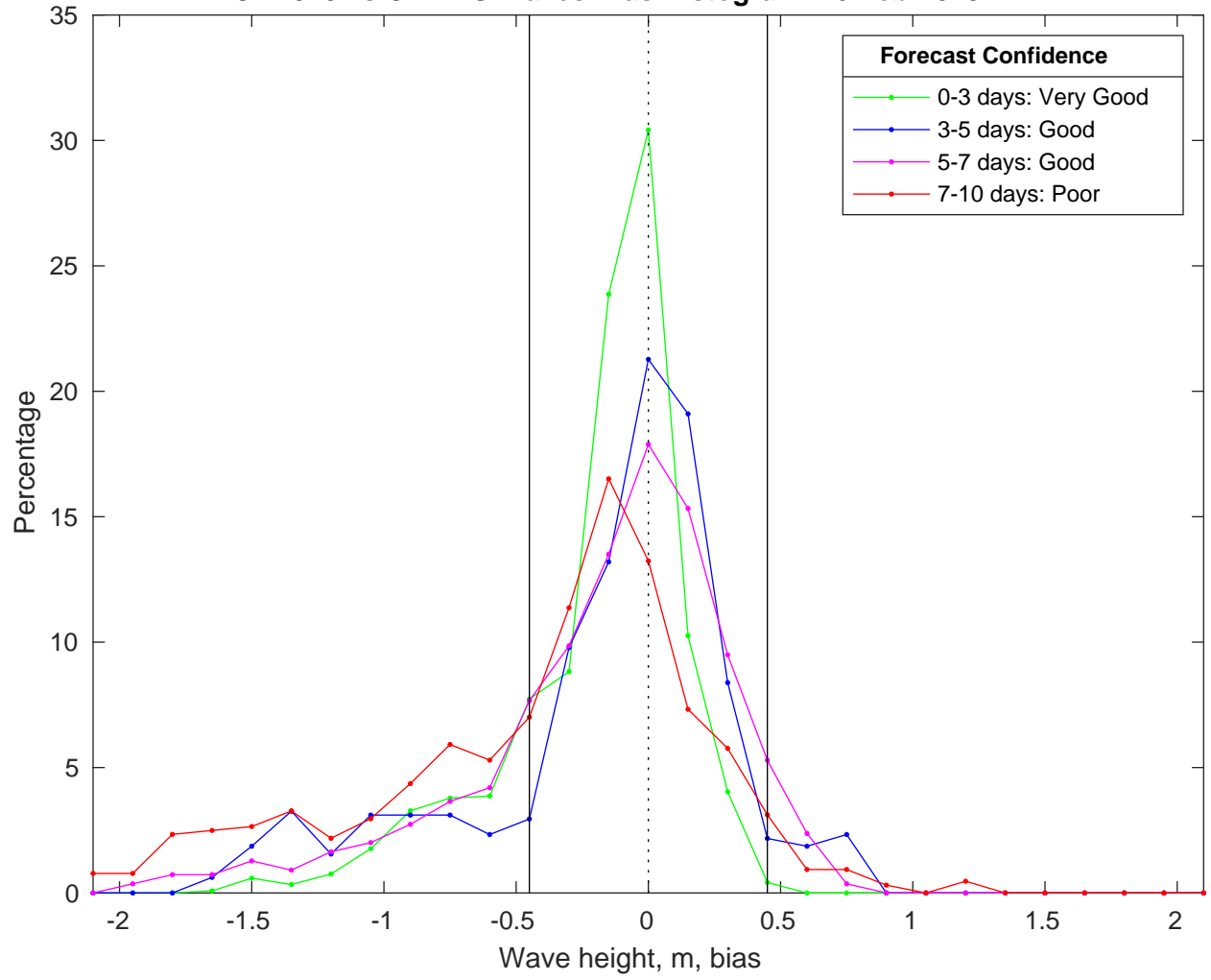
NDBC 42020 vs CMEMS Waves Bias Histogram: 26-Feb-2025
