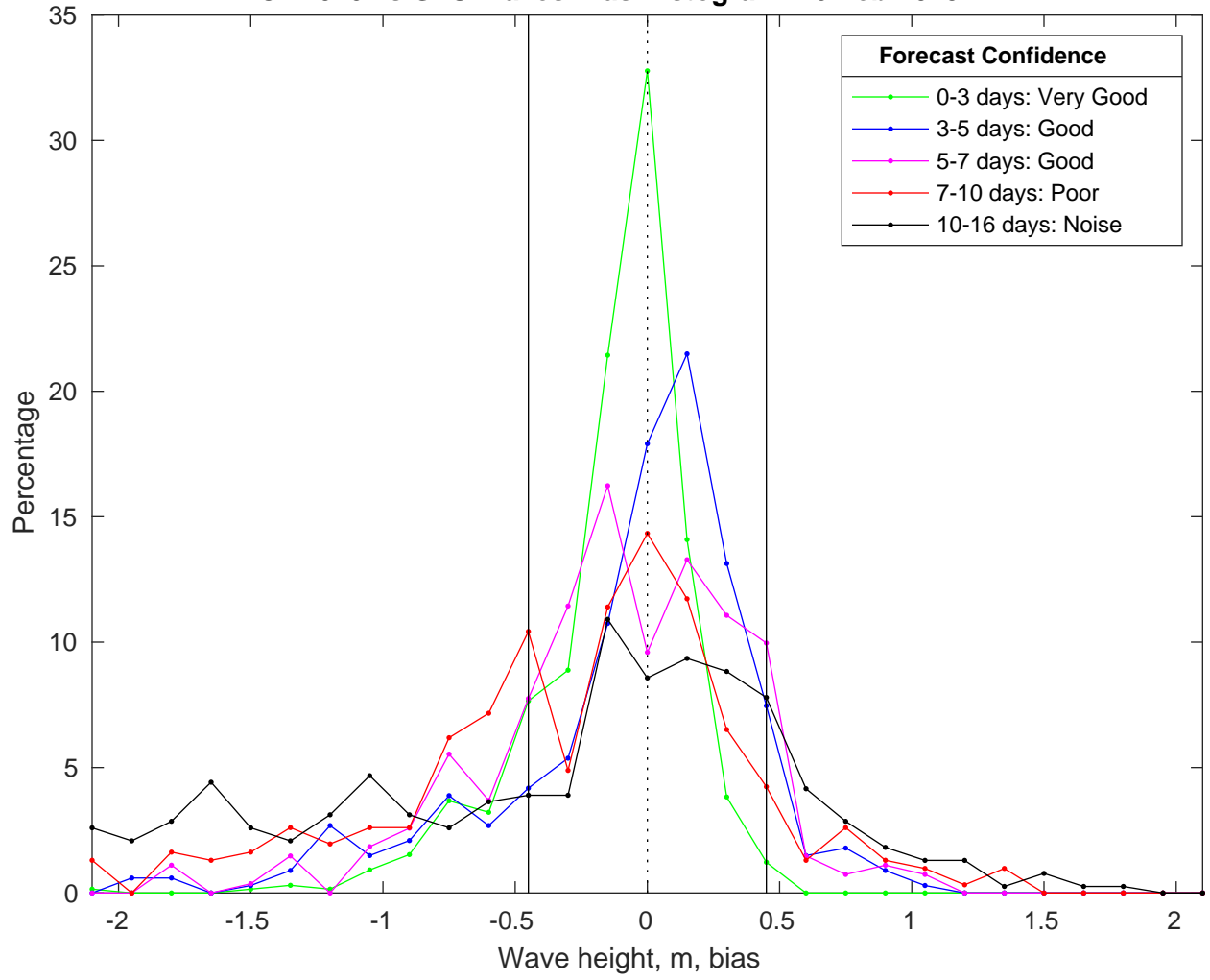
NDBC 42020 vs GFS Waves Bias Histogram: 26-Feb-2025
