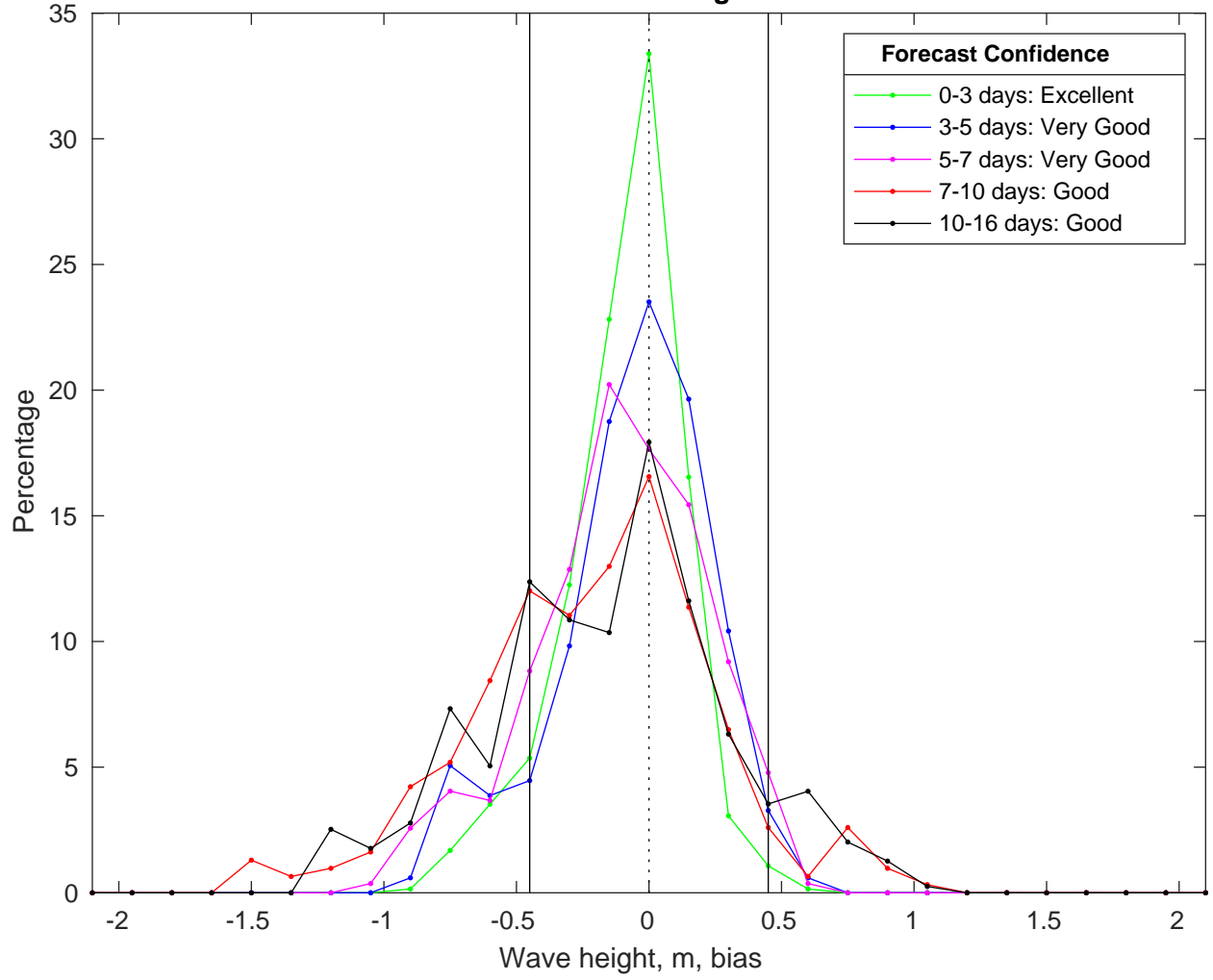
NDBC 42035 vs GFS Waves Bias Histogram: 26-Feb-2025
