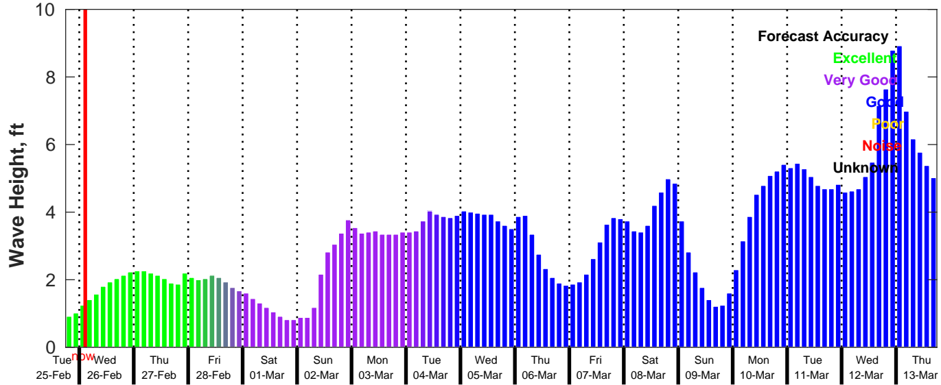
GFS Wave Forecast for NDBC 42035 from 25-Feb-2025 18:00:00 to 13-Mar-2025 18:00:00
