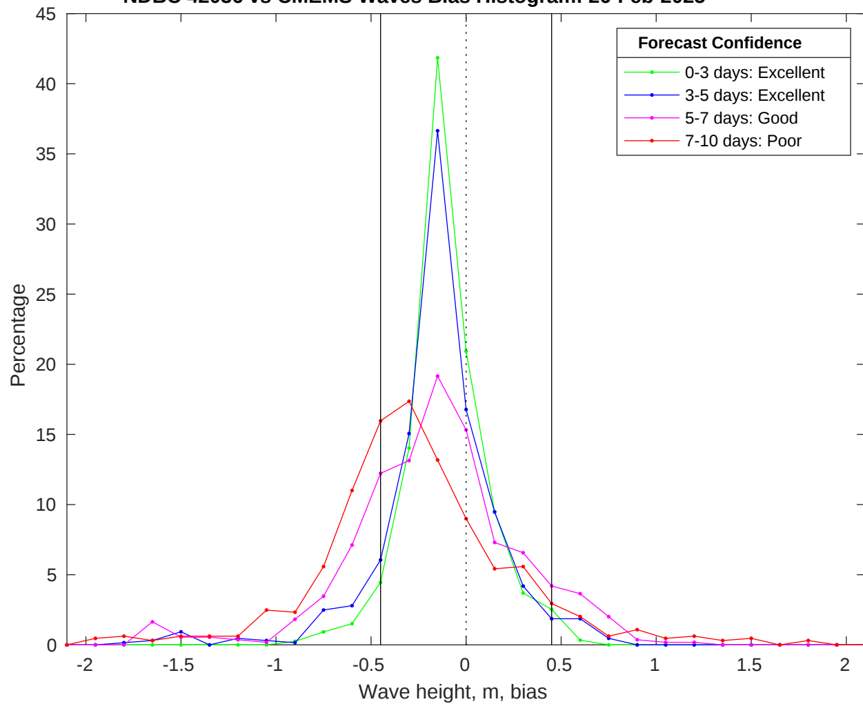
NDBC 42036 vs CMEMS Waves Bias Histogram: 26-Feb-2025
