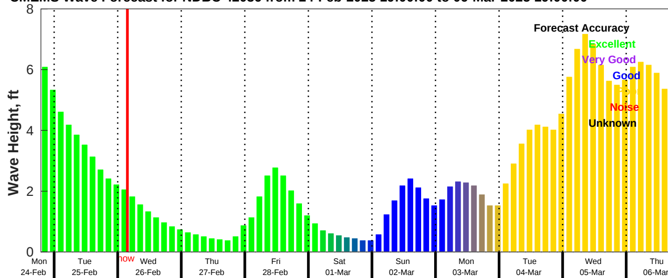
CMEMS Wave Forecast for NDBC 42036 from 24-Feb-2025 19:00:00 to 06-Mar-2025 19:00:00
