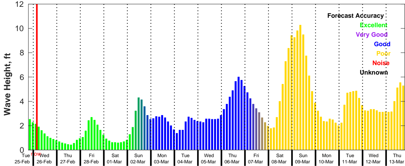
GFS Wave Forecast for NDBC 42036 from 25-Feb-2025 19:00:00 to 13-Mar-2025 19:00:00
