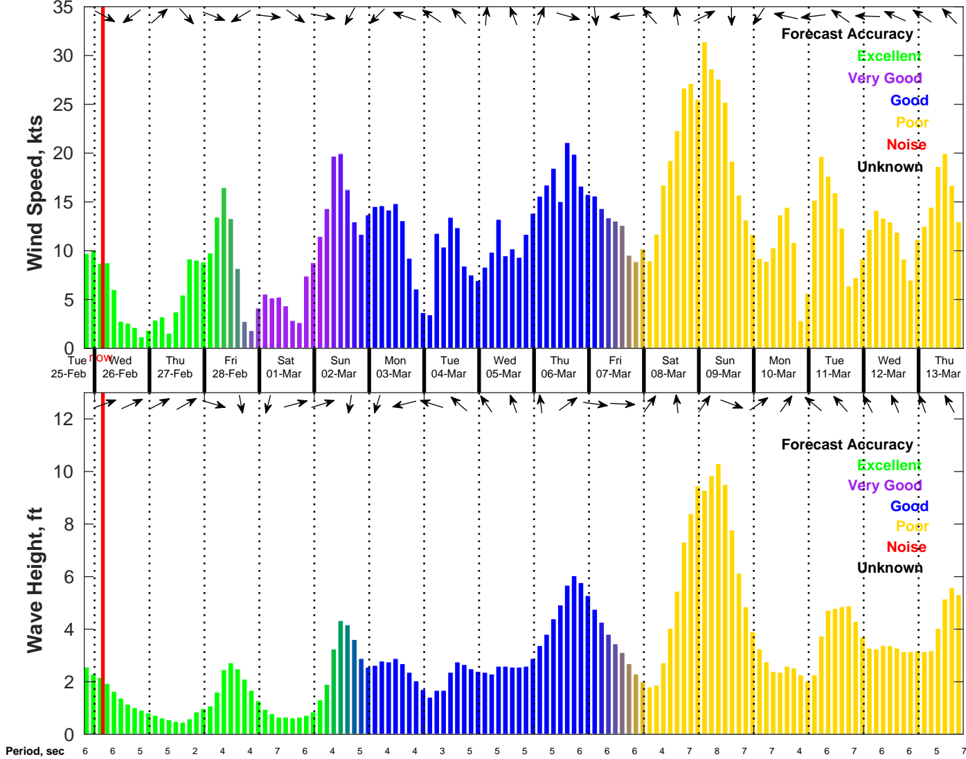
Wind & Wave Forecast for NDBC 42036 from 25-Feb-2025 19:00:00 to 13-Mar-2025 19:00:00
