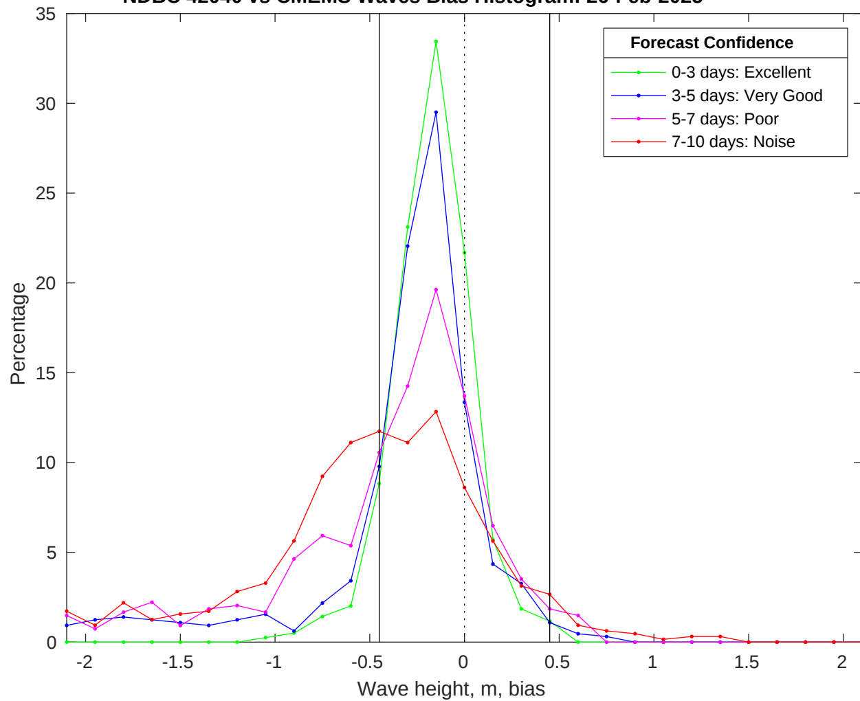
NDBC 42040 vs CMEMS Waves Bias Histogram: 26-Feb-2025
