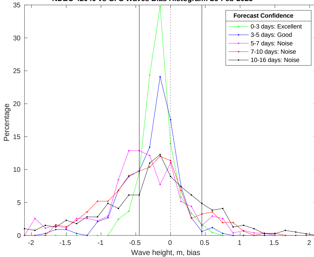
NDBC 42040 vs GFS Waves Bias Histogram: 26-Feb-2025
