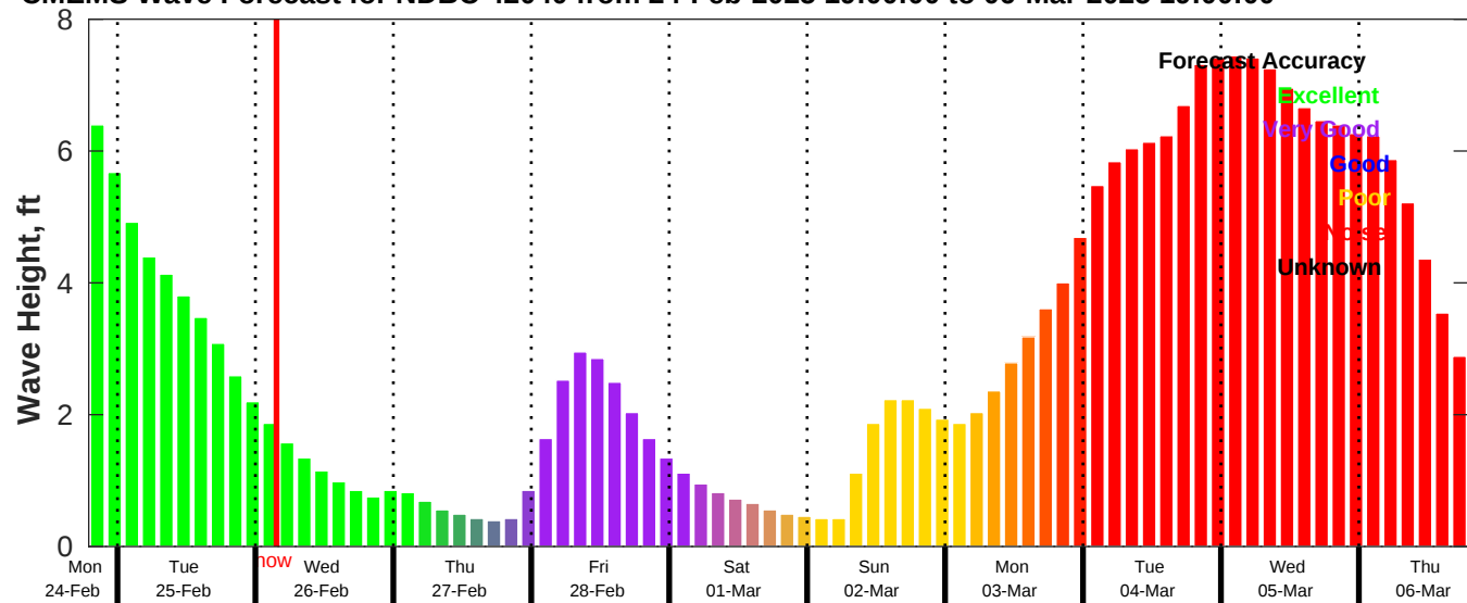
CMEMS Wave Forecast for NDBC 42040 from 24-Feb-2025 19:00:00 to 06-Mar-2025 19:00:00
