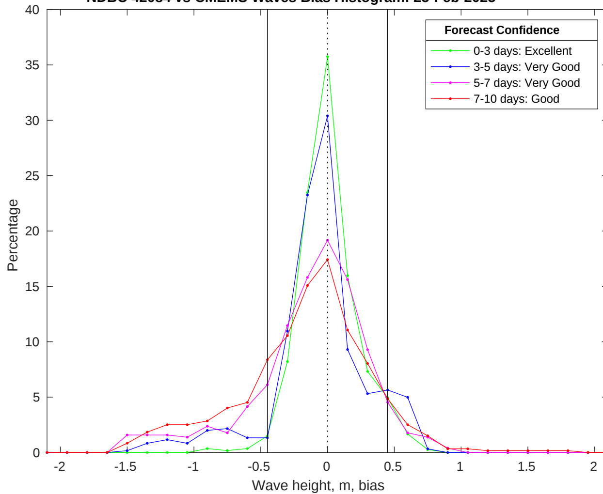
NDBC 42084 vs CMEMS Waves Bias Histogram: 25-Feb-2025
