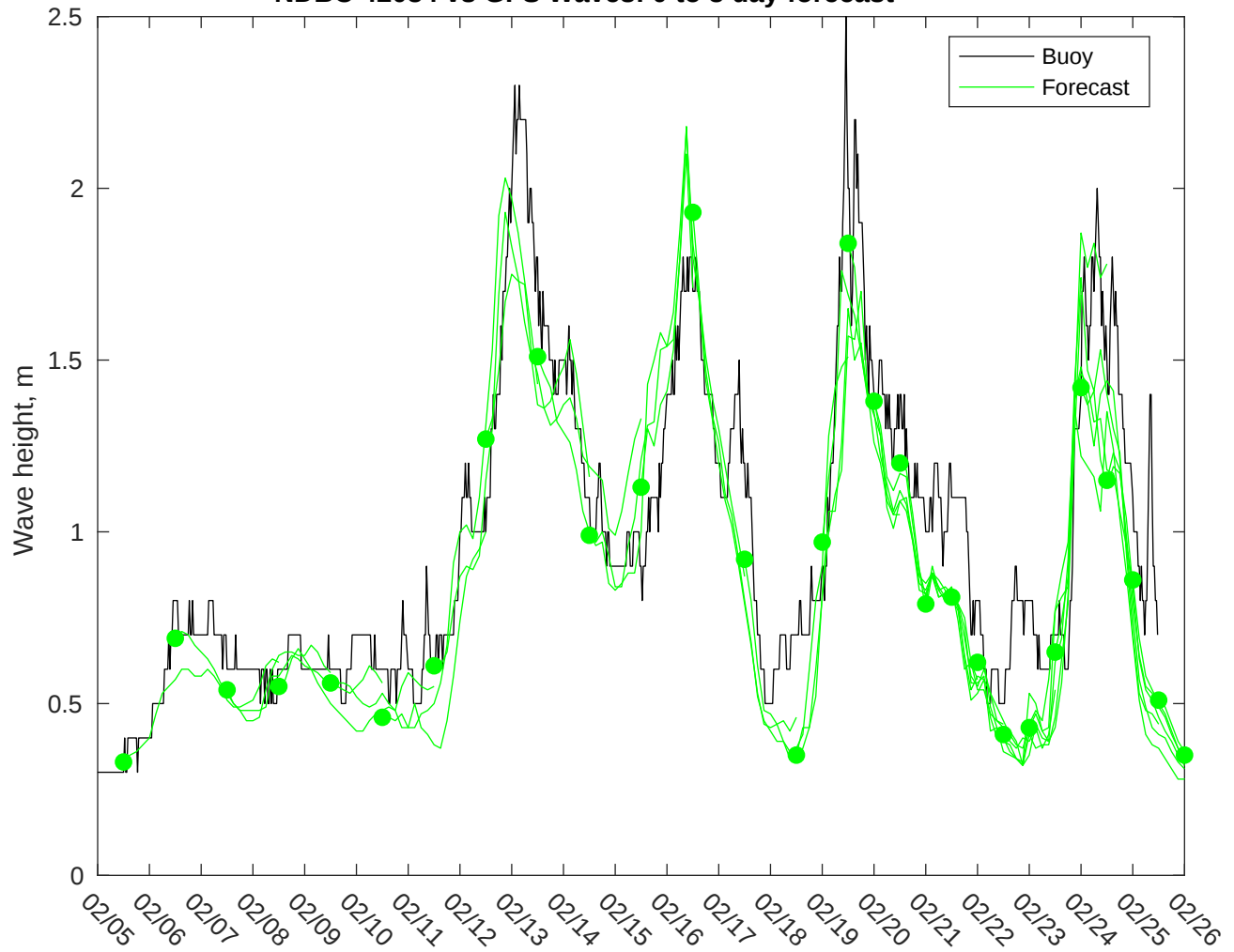
NDBC 42084 vs GFS Waves: 0 to 3 day forecast
