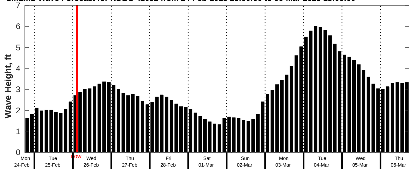
CMEMS Wave Forecast for NDBC 42092 from 24-Feb-2025 18:00:00 to 06-Mar-2025 18:00:00
