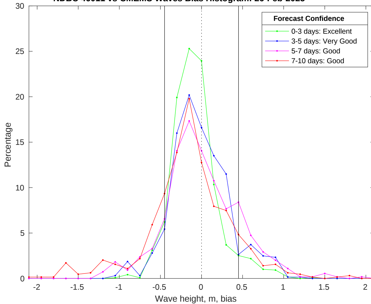
NDBC 46011 vs CMEMS Waves Bias Histogram: 26-Feb-2025
