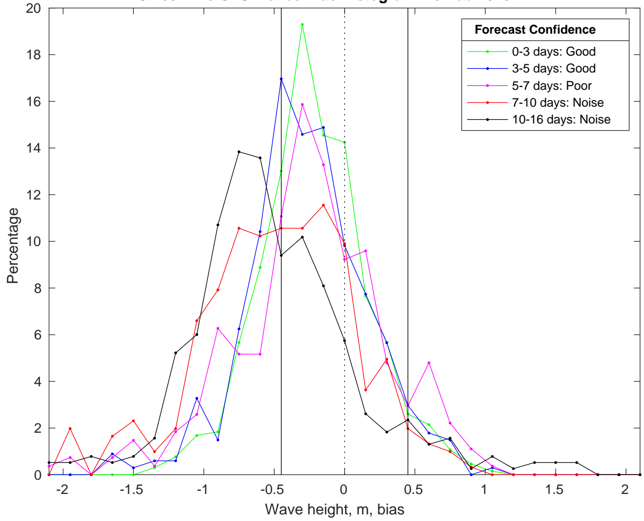
NDBC 46011 vs GFS Waves Bias Histogram: 26-Feb-2025
