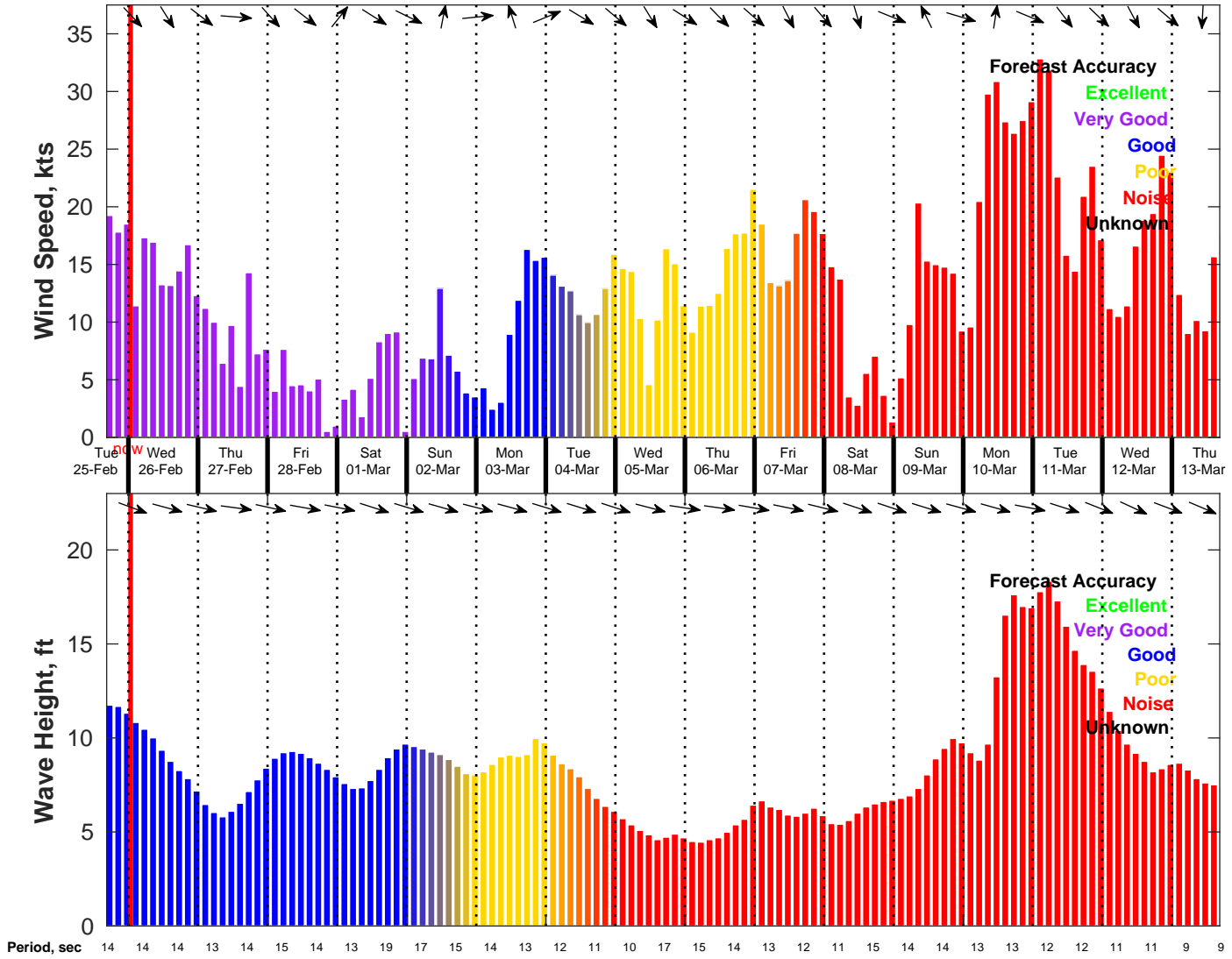
Wind & Wave Forecast for NDBC 46011 from 25-Feb-2025 16:00:00 to 13-Mar-2025 16:00:00
