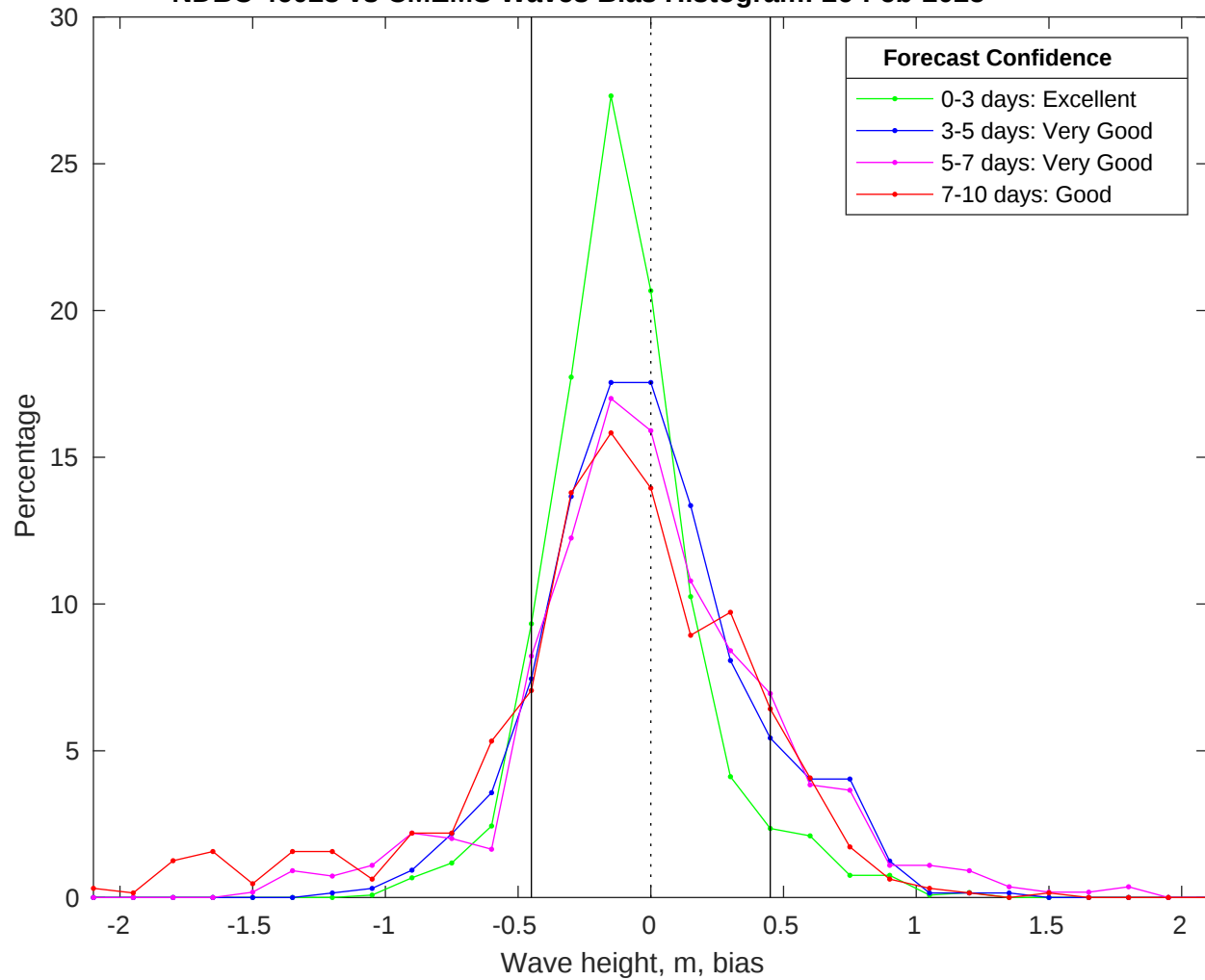
NDBC 46028 vs CMEMS Waves Bias Histogram: 26-Feb-2025
