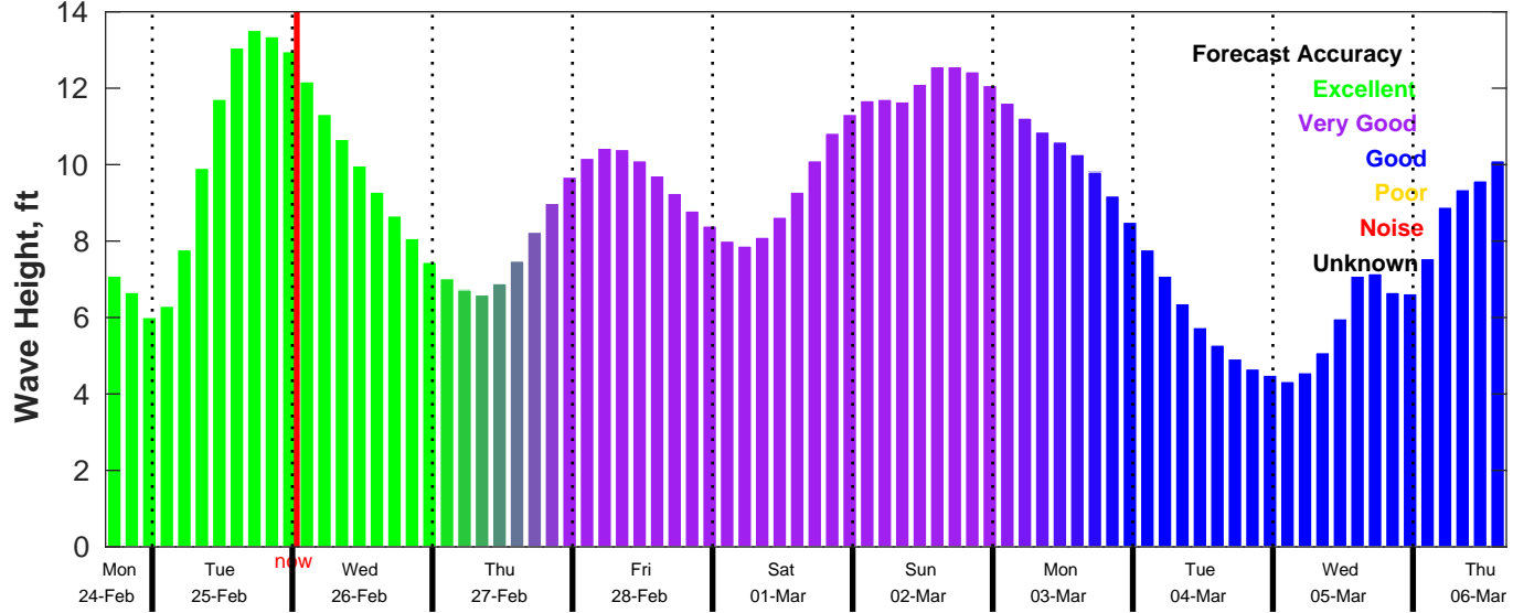
CMEMS Wave Forecast for NDBC 46028 from 24-Feb-2025 16:00:00 to 06-Mar-2025 16:00:00
