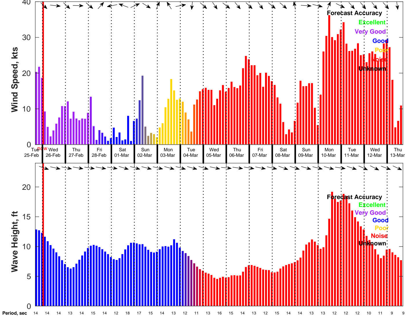
Wind & Wave Forecast for NDBC 46028 from 25-Feb-2025 16:00:00 to 13-Mar-2025 16:00:00
