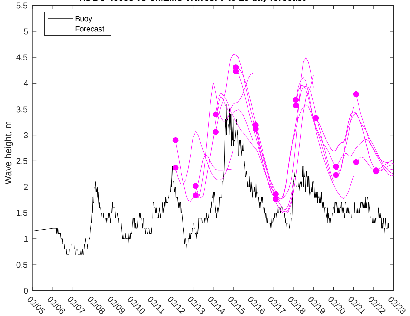
NDBC 46053 vs CMEMS Waves: 7 to 10 day forecast
