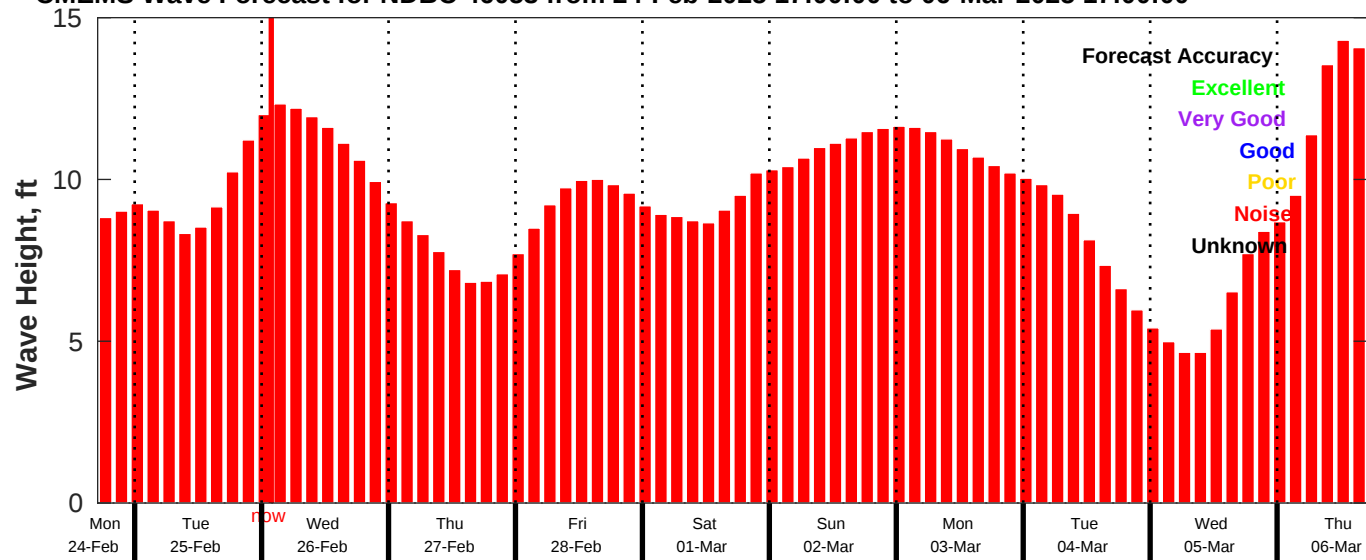
CMEMS Wave Forecast for NDBC 46053 from 24-Feb-2025 17:00:00 to 06-Mar-2025 17:00:00
