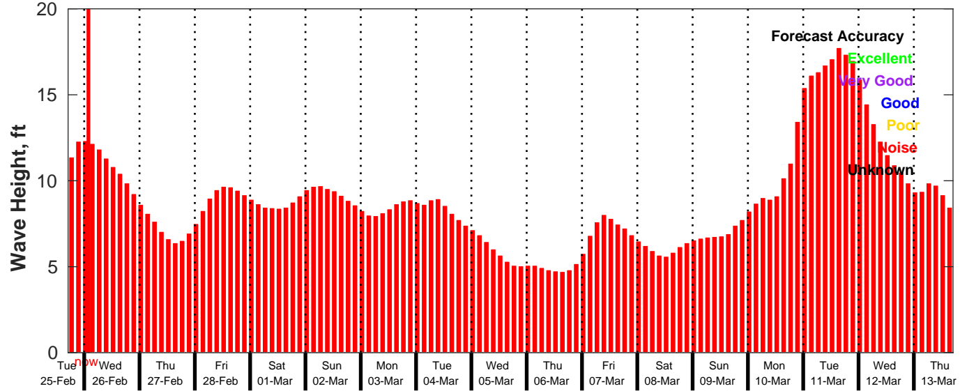
GFS Wave Forecast for NDBC 46053 from 25-Feb-2025 17:00:00 to 13-Mar-2025 17:00:00
