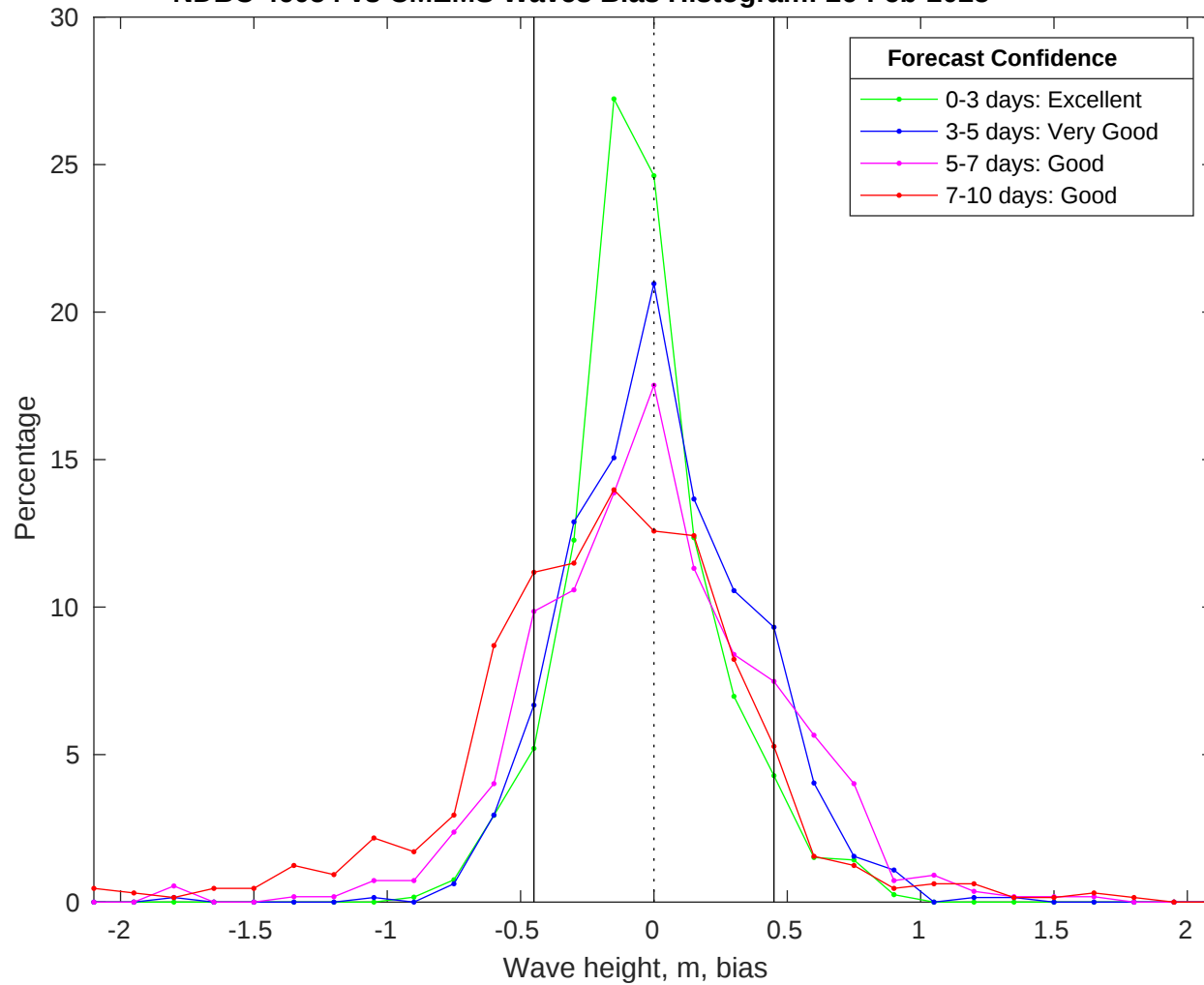
NDBC 46054 vs CMEMS Waves Bias Histogram: 26-Feb-2025
