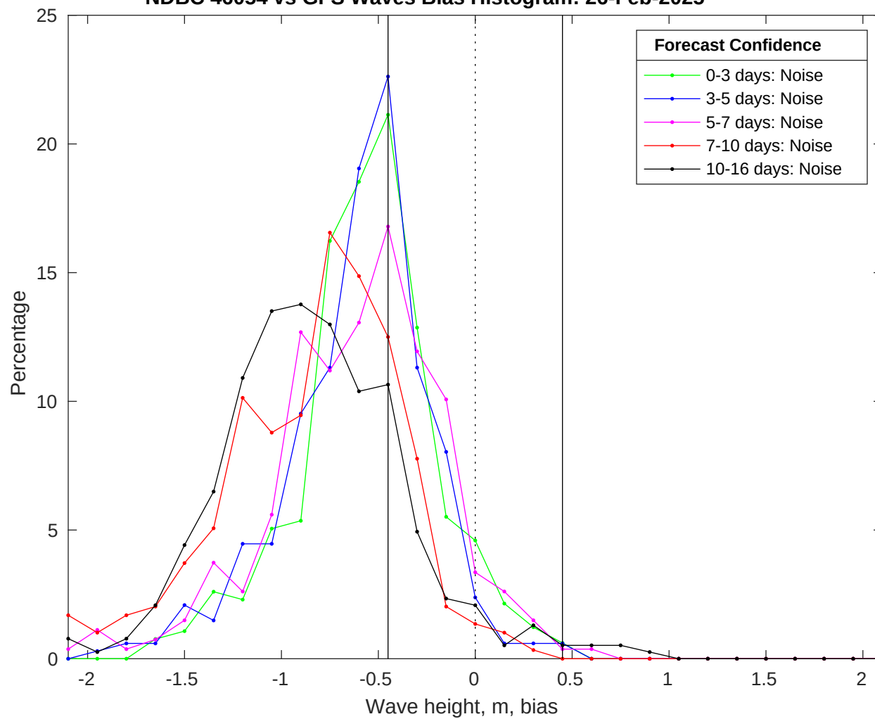
NDBC 46054 vs GFS Waves Bias Histogram: 26-Feb-2025
