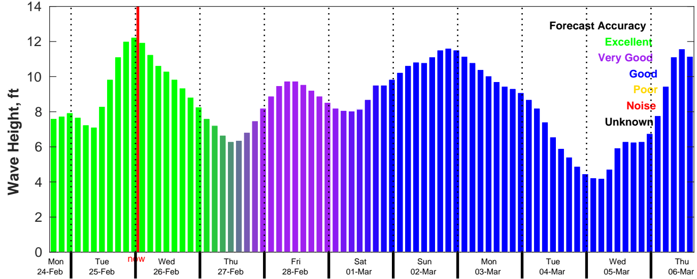
CMEMS Wave Forecast for NDBC 46054 from 24-Feb-2025 16:00:00 to 06-Mar-2025 16:00:00
