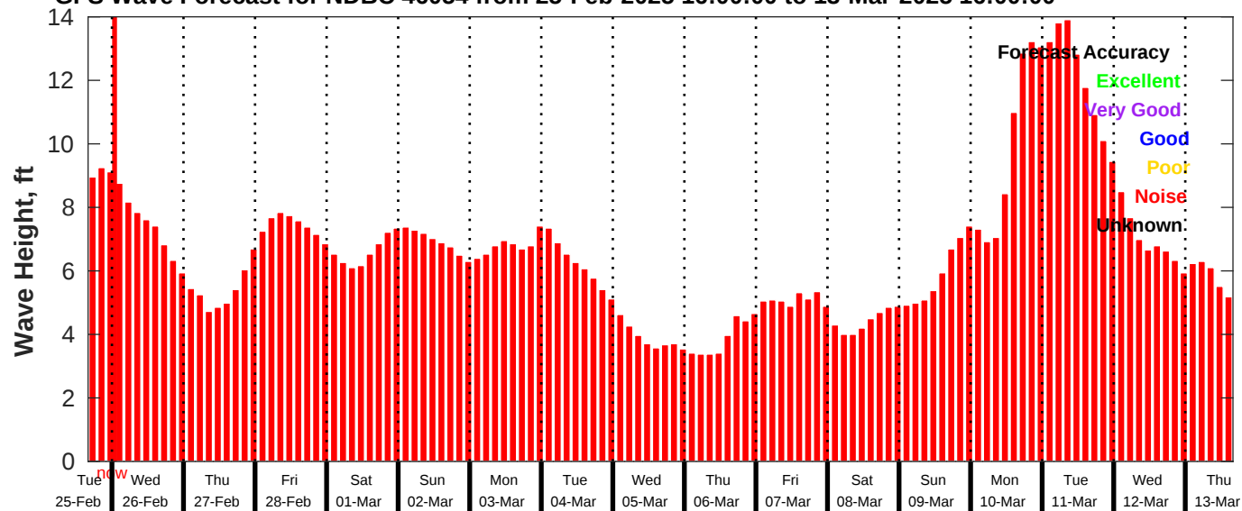
GFS Wave Forecast for NDBC 46054 from 25-Feb-2025 16:00:00 to 13-Mar-2025 16:00:00
