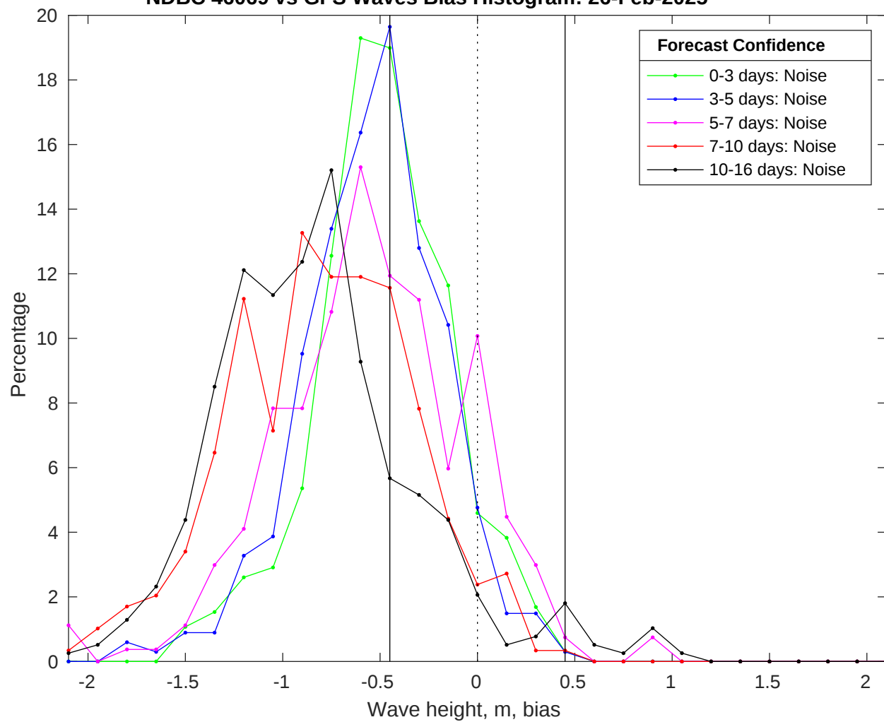
NDBC 46069 vs GFS Waves Bias Histogram: 26-Feb-2025
